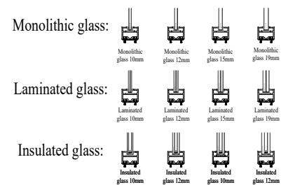
Glass fitting diagram
