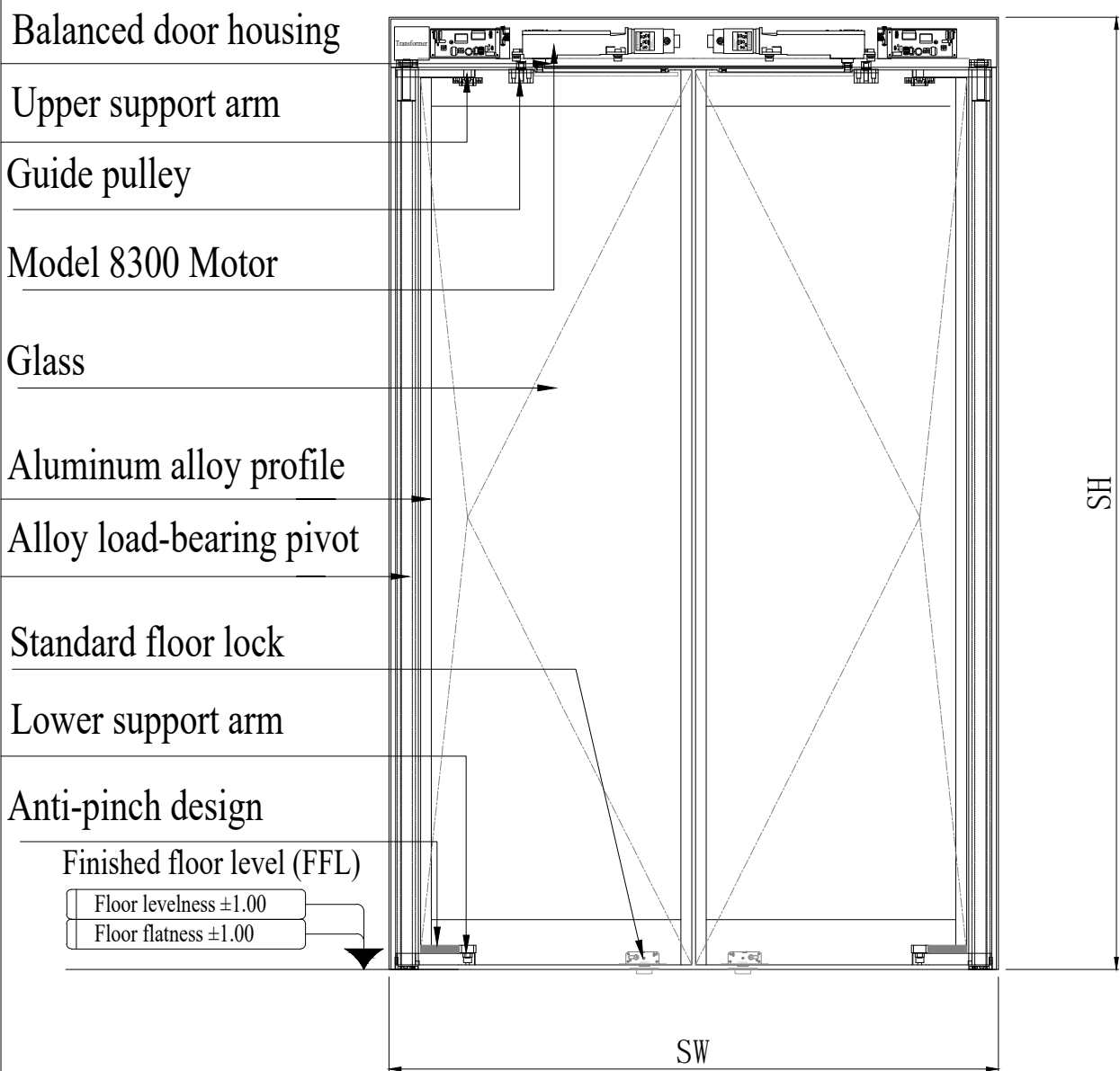
Elevation view
