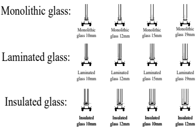
Glass fitting diagram
